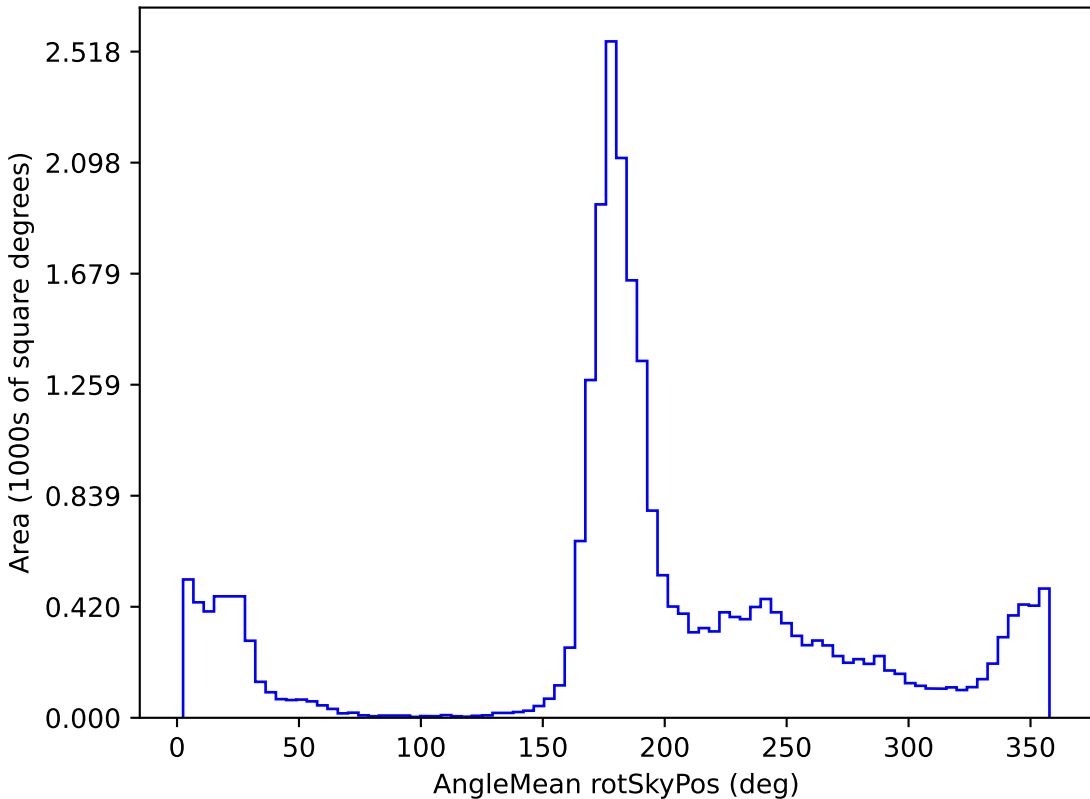
too_100_4v3.4_10yrs All sky r band: AngleMean rotSkyPos
