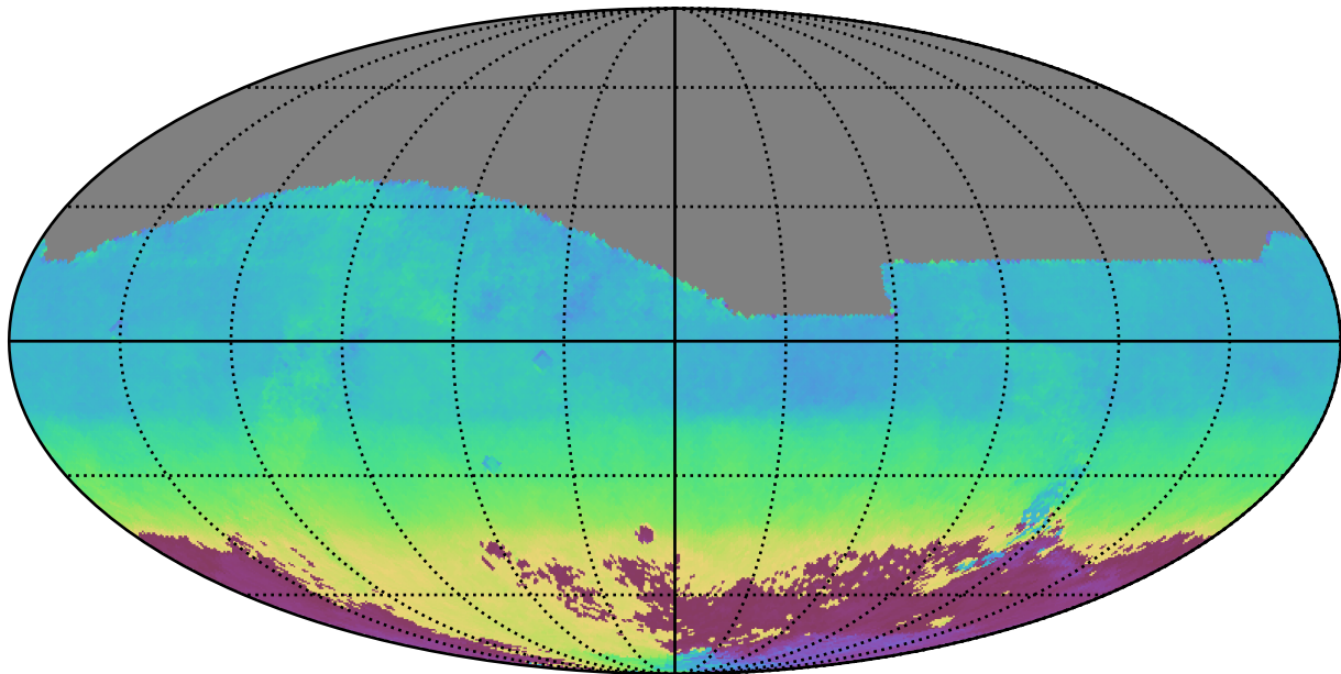
too_100_4v3.4_10yrs All sky i band: AngleMean rotSkyPos
