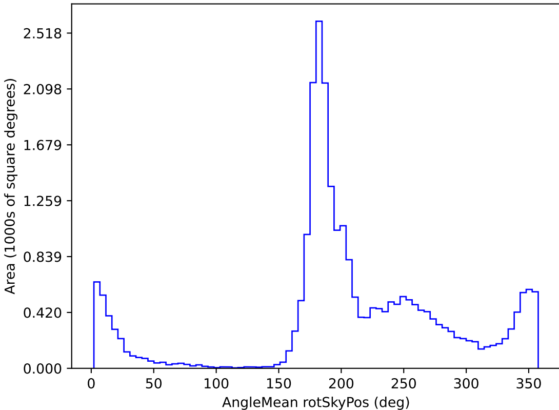
too_100_4v3.4_10yrs All sky i band: AngleMean rotSkyPos
