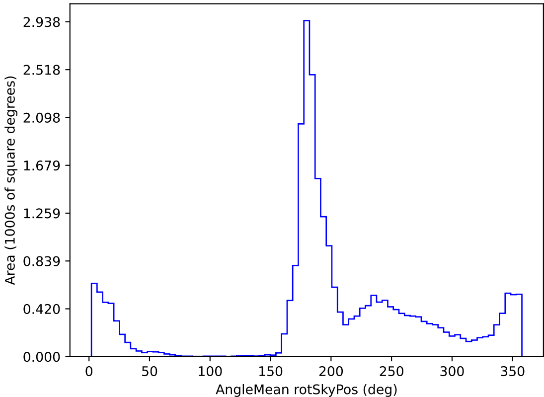
too_100_4v3.4_10yrs All sky all bands: AngleMean rotSkyPos
