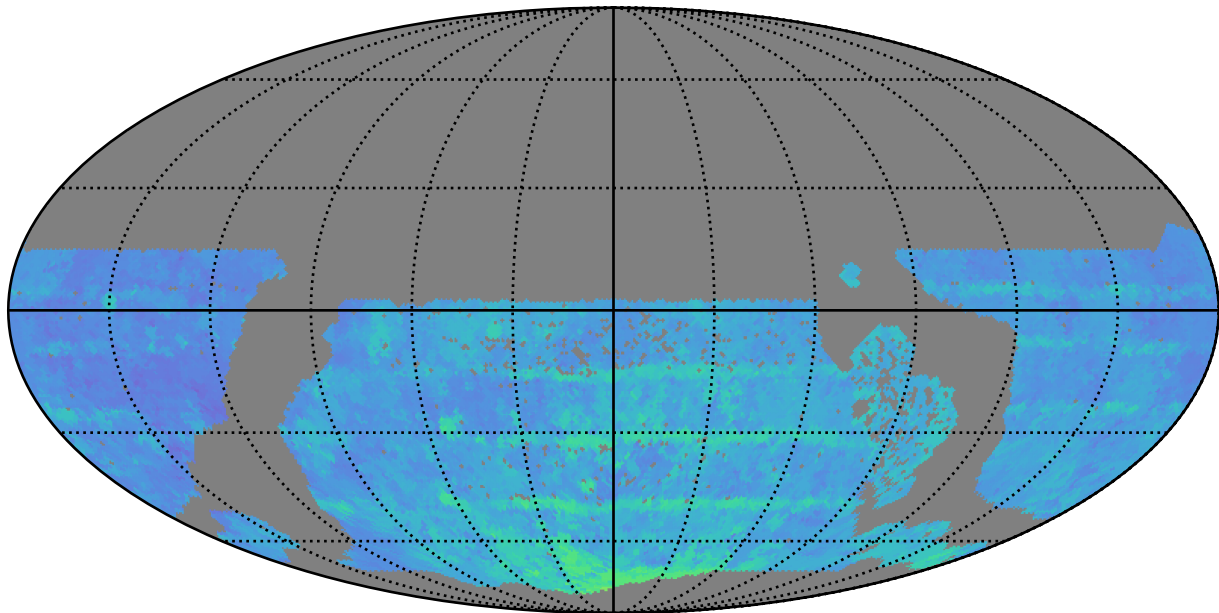
too_100_4v3.4_10yrs WFD z band: 80thPercentile Season Length
