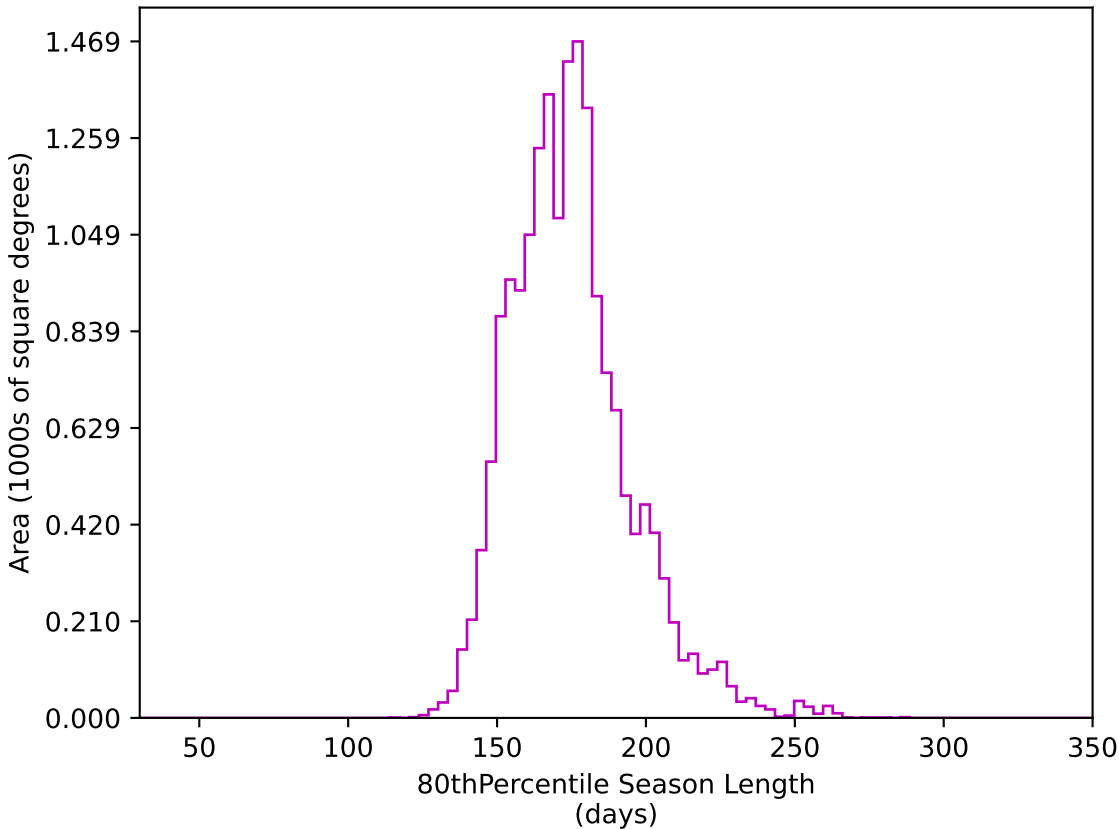
too_100_4v3.4_10yrs WFD z band: 80thPercentile Season Length
