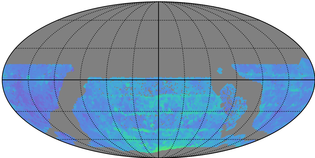
too_100_4v3.4_10yrs WFD y band: 80thPercentile Season Length
