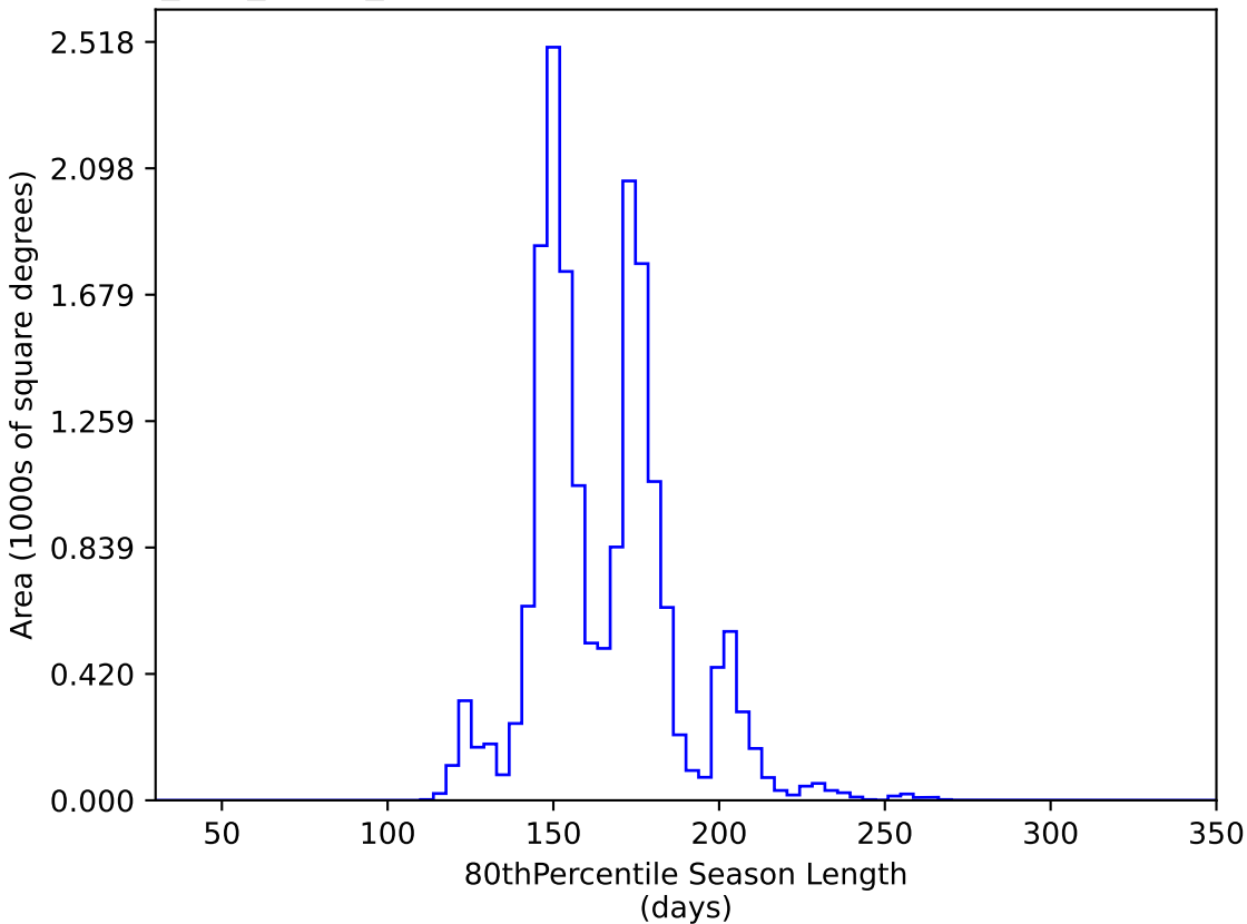
too_100_4v3.4_10yrs WFD y band: 80thPercentile Season Length
