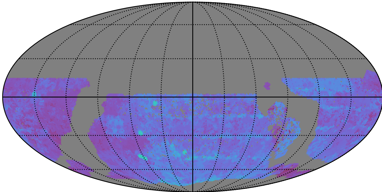
too_100_4v3.4_10yrs WFD u band: 80thPercentile Season Length
