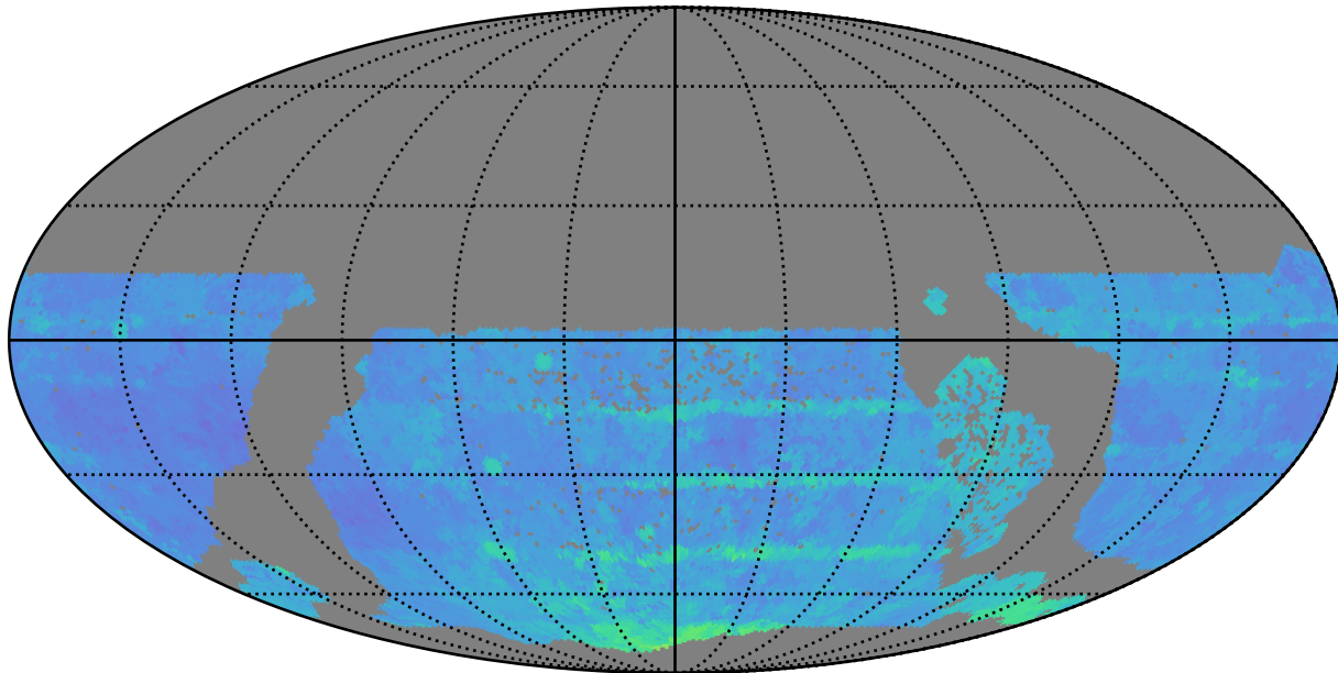
too_100_4v3.4_10yrs WFD r band: 80thPercentile Season Length
