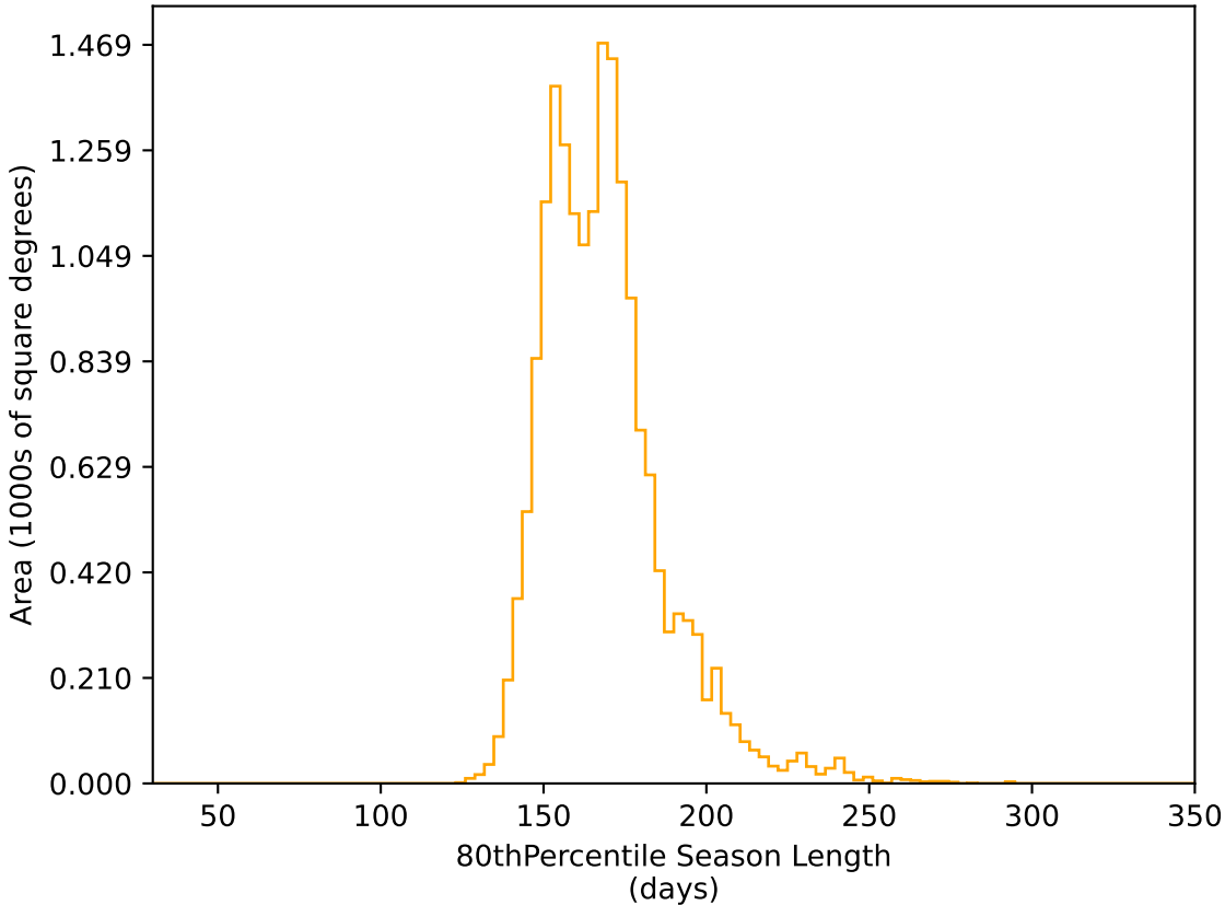
too_100_4v3.4_10yrs WFD r band: 80thPercentile Season Length
