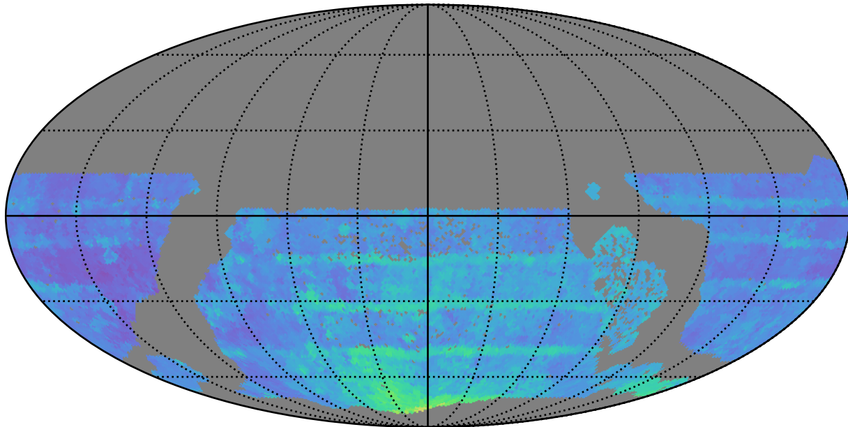
too_100_4v3.4_10yrs WFD all bands: 80thPercentile Season Length
