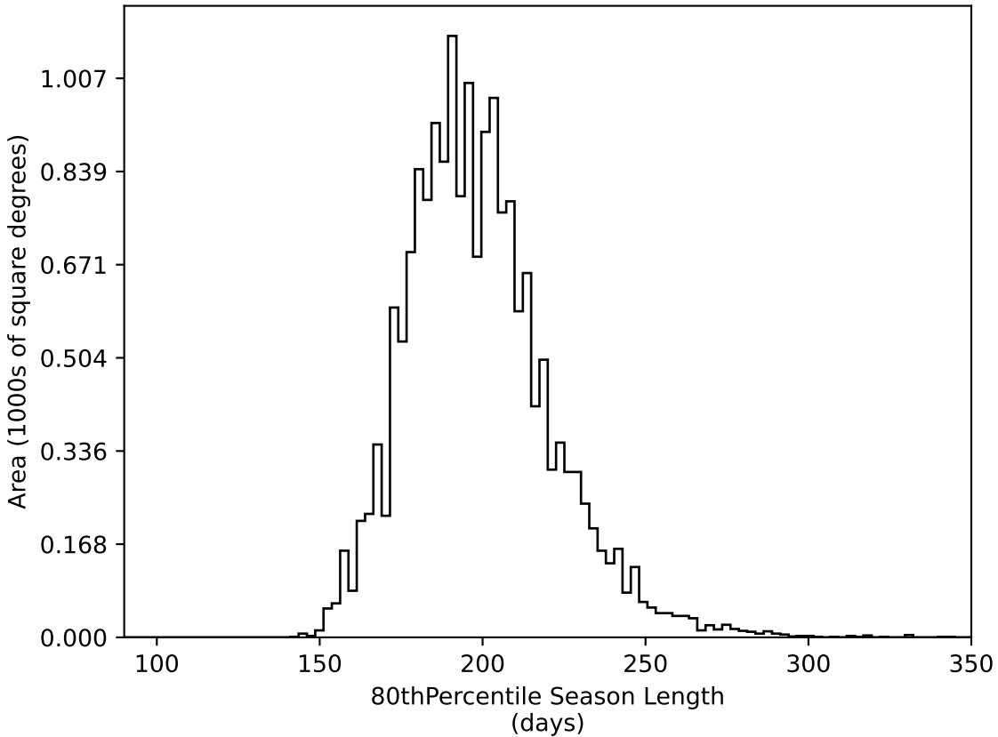
too_100_4v3.4_10yrs WFD all bands: 80thPercentile Season Length
