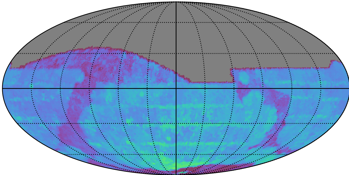
too_100_4v3.4_10yrs All sky z band: 80thPercentile Season Length
