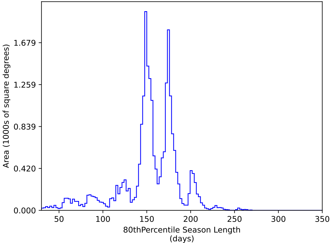
too_100_4v3.4_10yrs All sky y band: 80thPercentile Season Length
