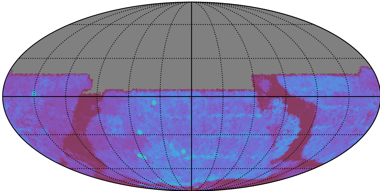
too_100_4v3.4_10yrs All sky u band: 80thPercentile Season Length
