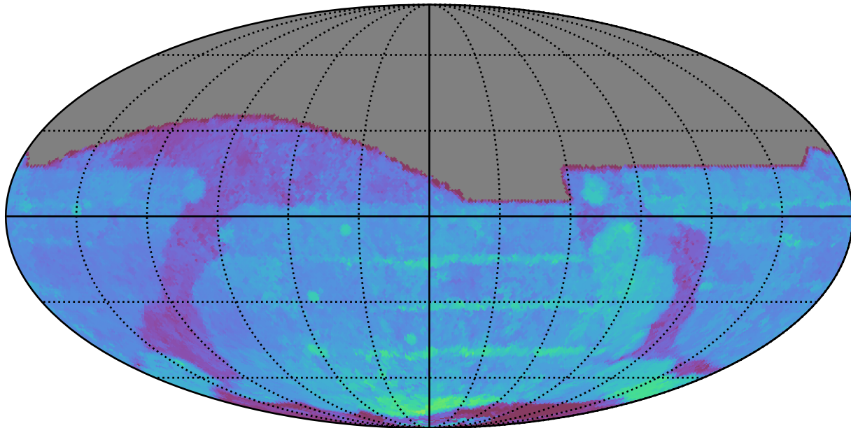
too_100_4v3.4_10yrs All sky r band: 80thPercentile Season Length
