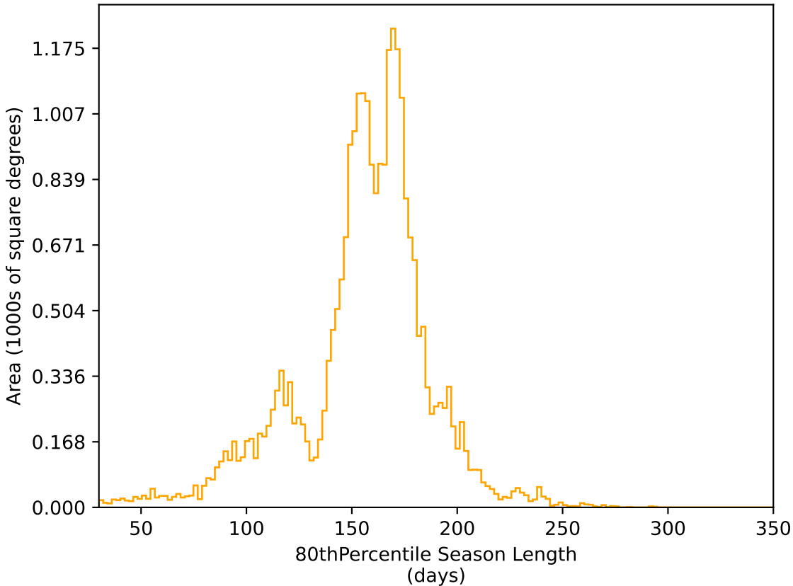
too_100_4v3.4_10yrs All sky r band: 80thPercentile Season Length
