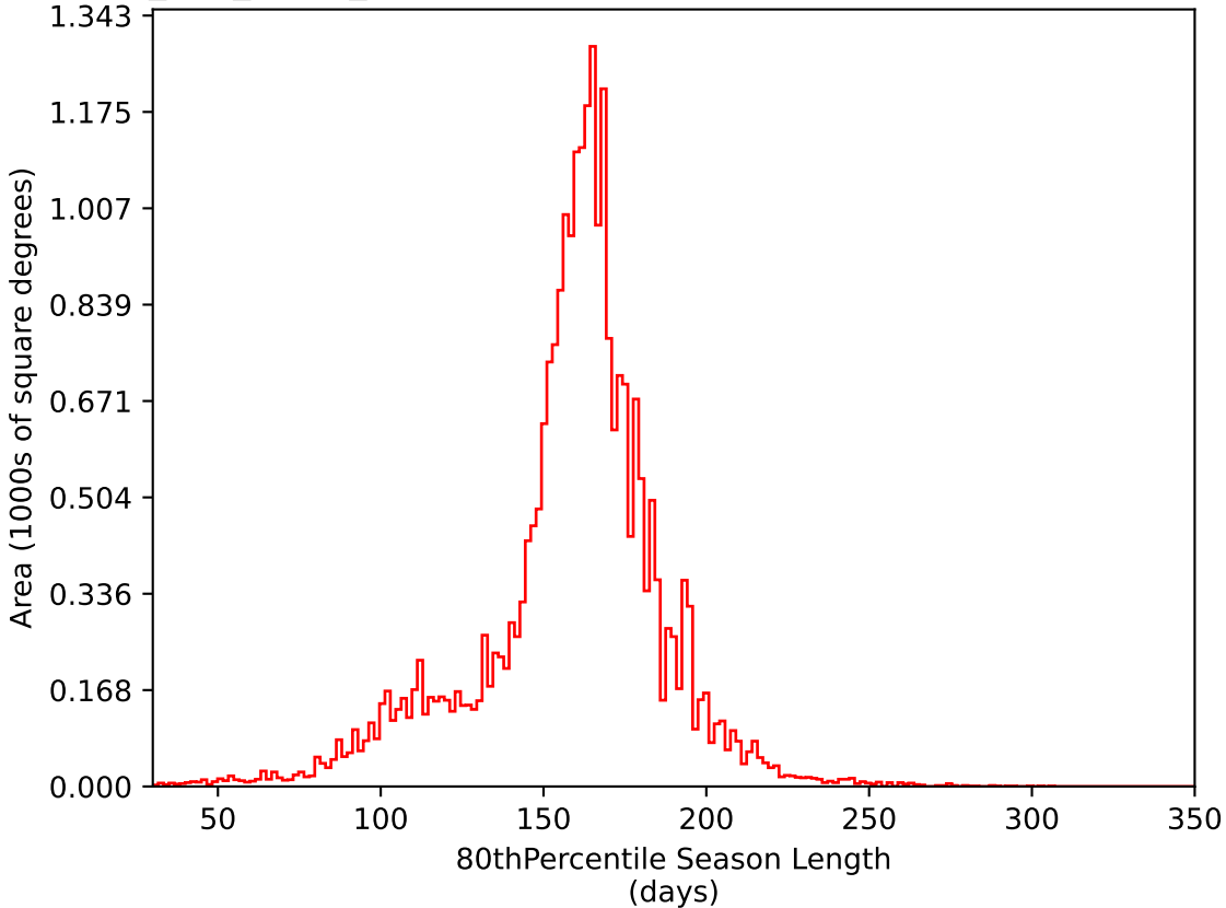
too_100_4v3.4_10yrs All sky i band: 80thPercentile Season Length
