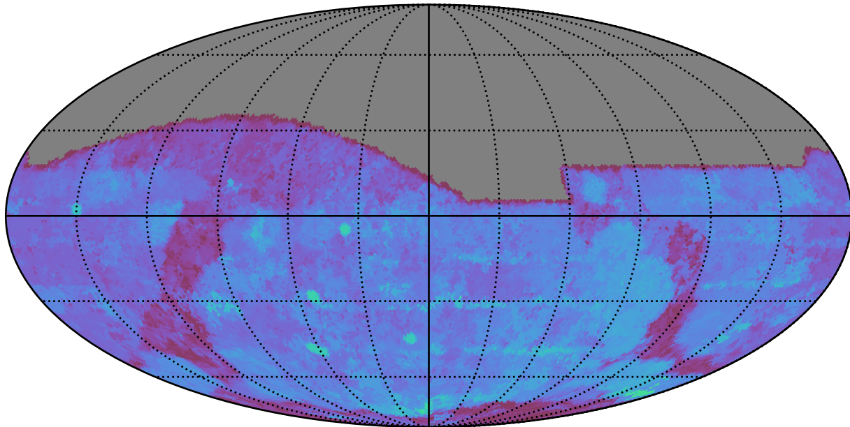
too_100_4v3.4_10yrs All sky g band: 80thPercentile Season Length
