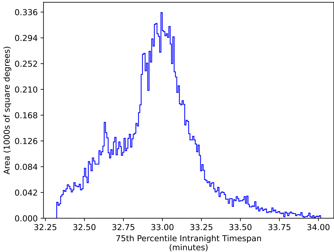
too_100_4v3.4_10yrs WFD y band: 75th Percentile Intranight Timespan
