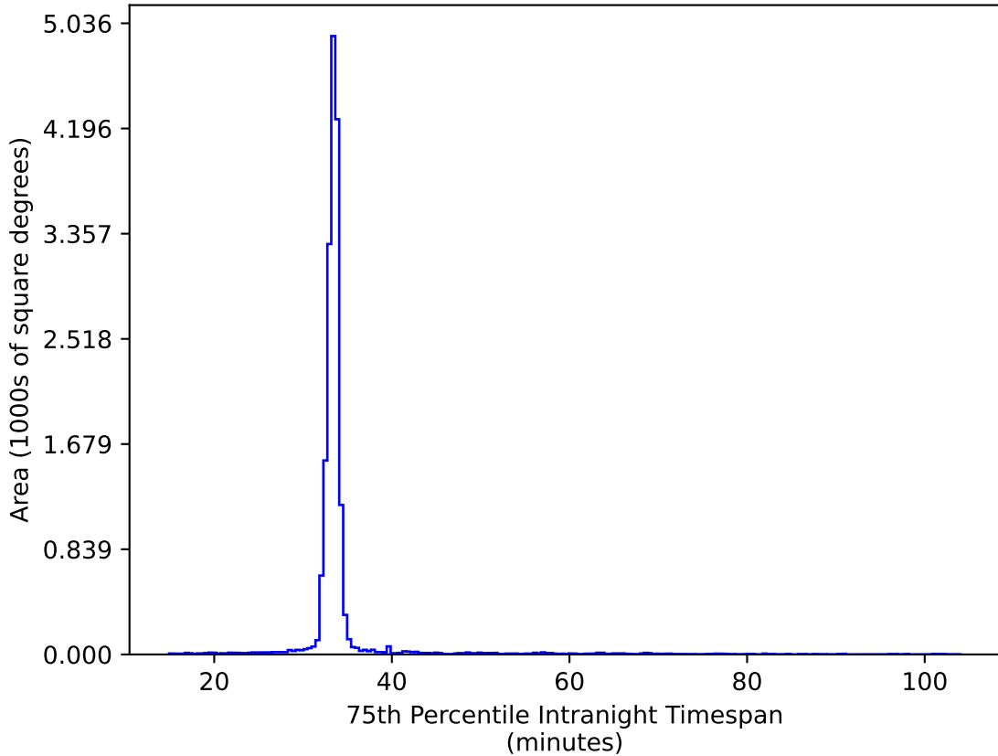
too_100_4v3.4_10yrs WFD ug bands: 75th Percentile Intranight Timespan
