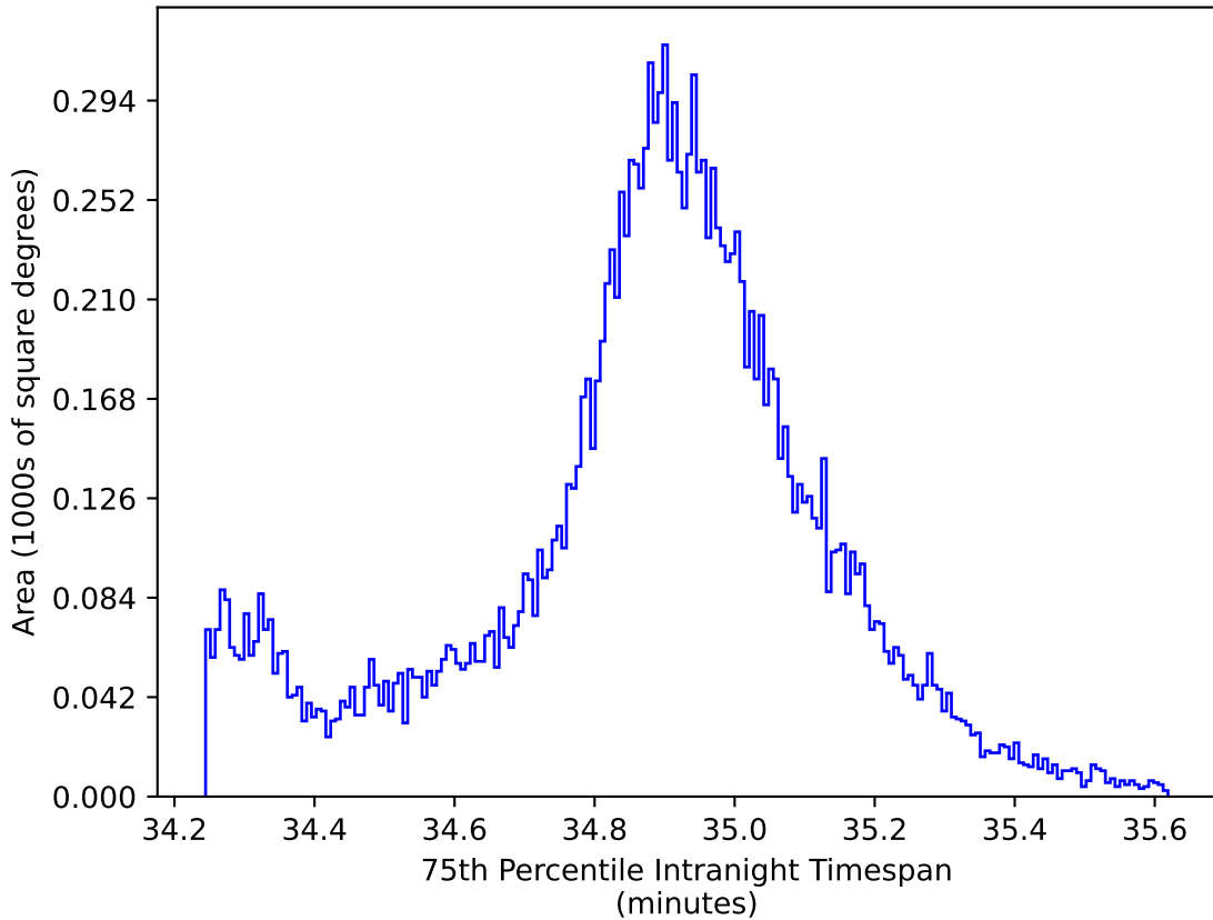
too_100_4v3.4_10yrs WFD all bands: 75th Percentile Intranight Timespan
