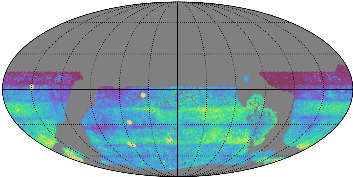
too_100_4v3.4_10yrs WFD: 75th Percentile Intranight Timespan
