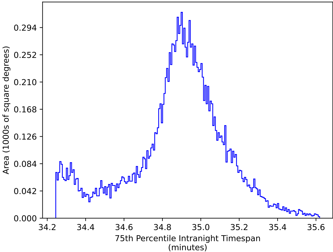
too_100_4v3.4_10yrs WFD: 75th Percentile Intranight Timespan
