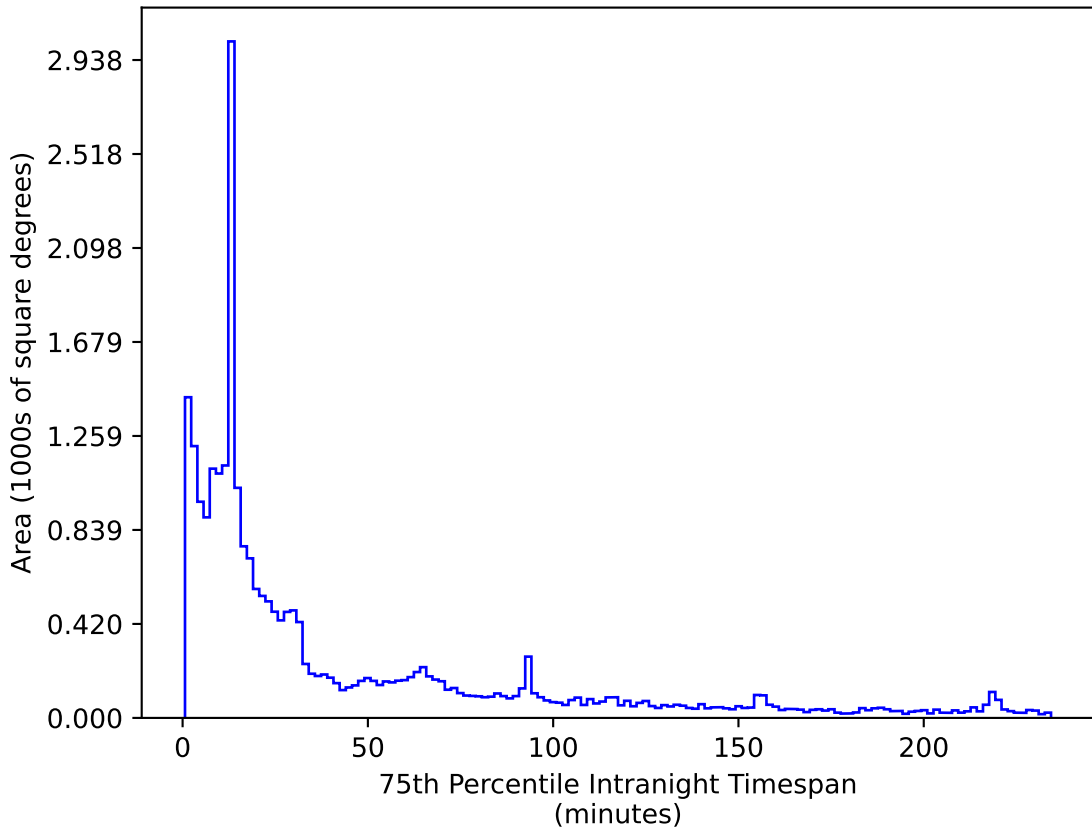
too_100_4v3.4_10yrs All sky z band: 75th Percentile Intranight Timespan
