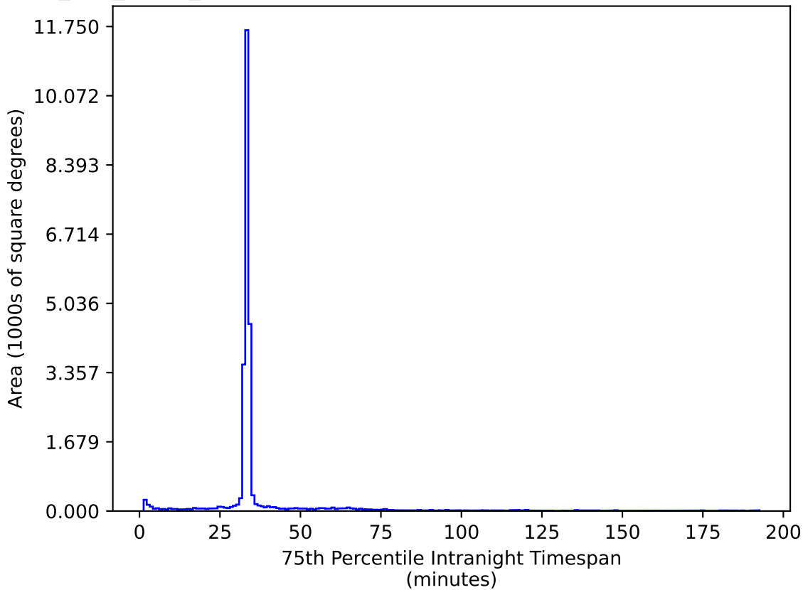
too_100_4v3.4_10yrs All sky ug bands: 75th Percentile Intranight Timespan
