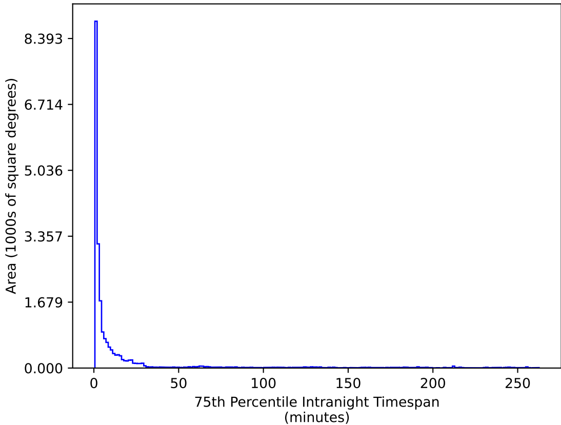
too_100_4v3.4_10yrs All sky u band: 75th Percentile Intranight Timespan
