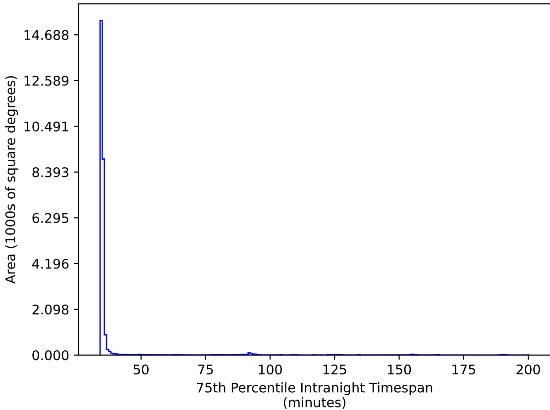
too_100_4v3.4_10yrs All sky ri bands: 75th Percentile Intranight Timespan
