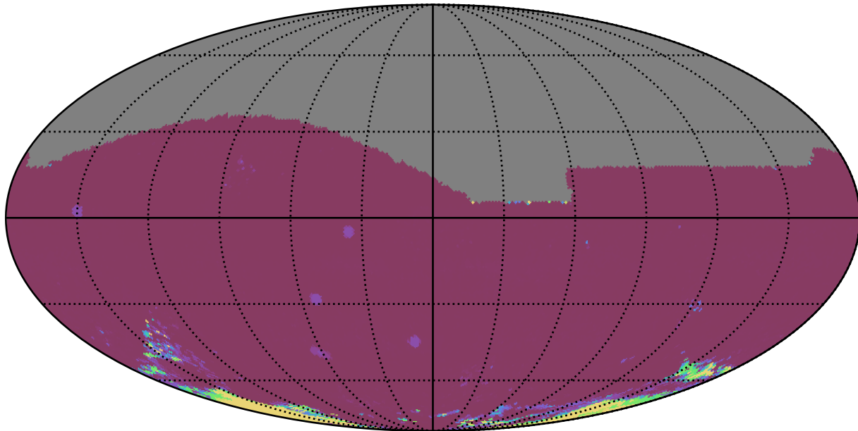
too_100_4v3.4_10yrs All sky iz bands: 75th Percentile Intranight Timespan
