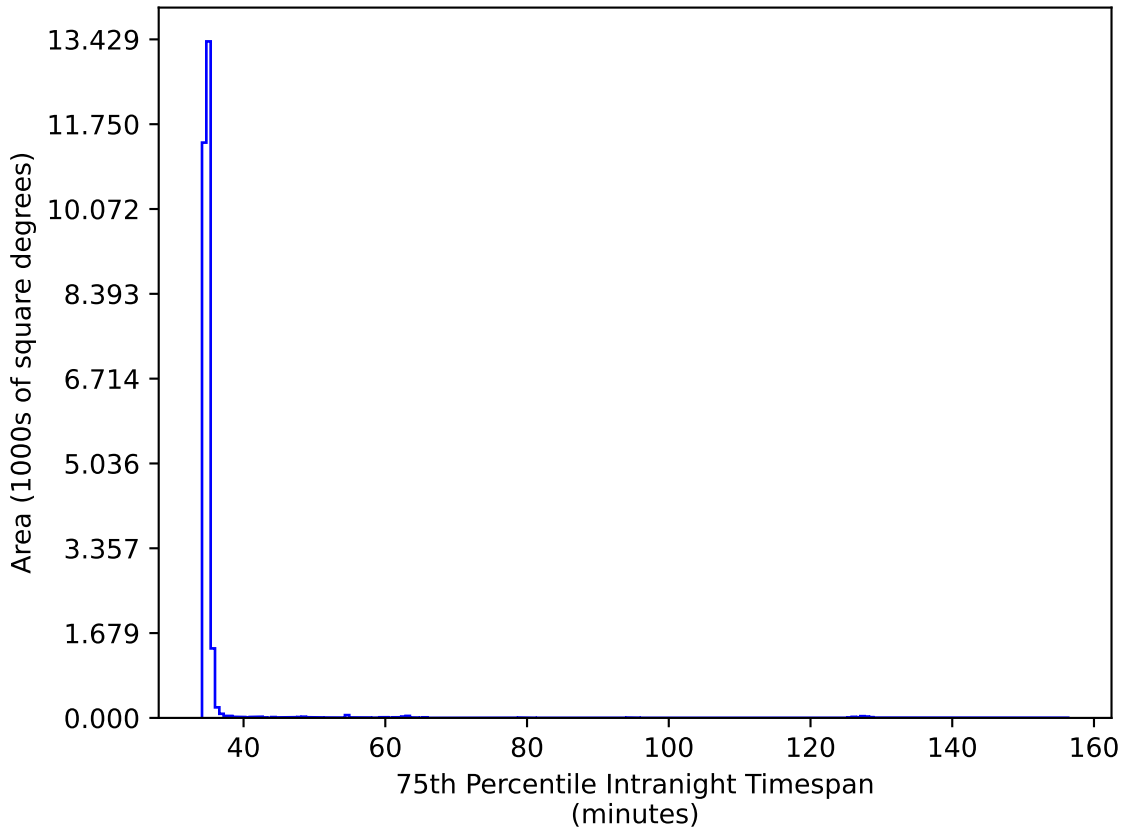
too_100_4v3.4_10yrs All sky iz bands: 75th Percentile Intranight Timespan
