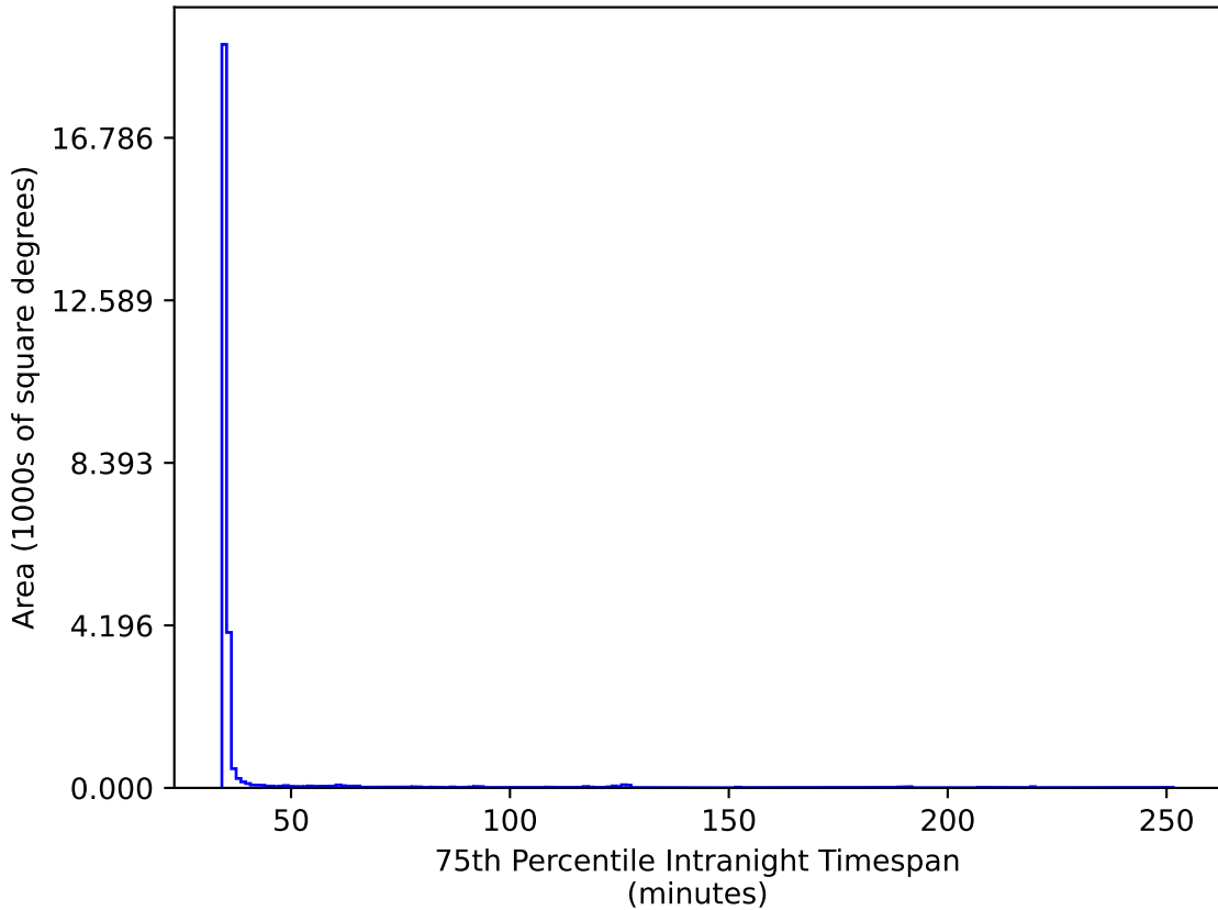
too_100_4v3.4_10yrs All sky gr bands: 75th Percentile Intranight Timespan
