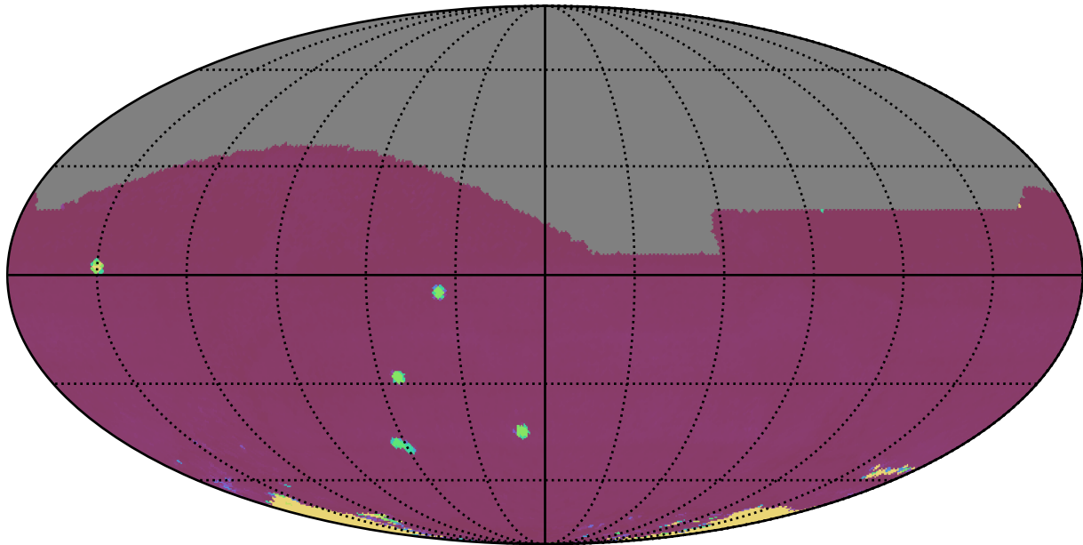
too_100_4v3.4_10yrs All sky: 75th Percentile Intranight Timespan
