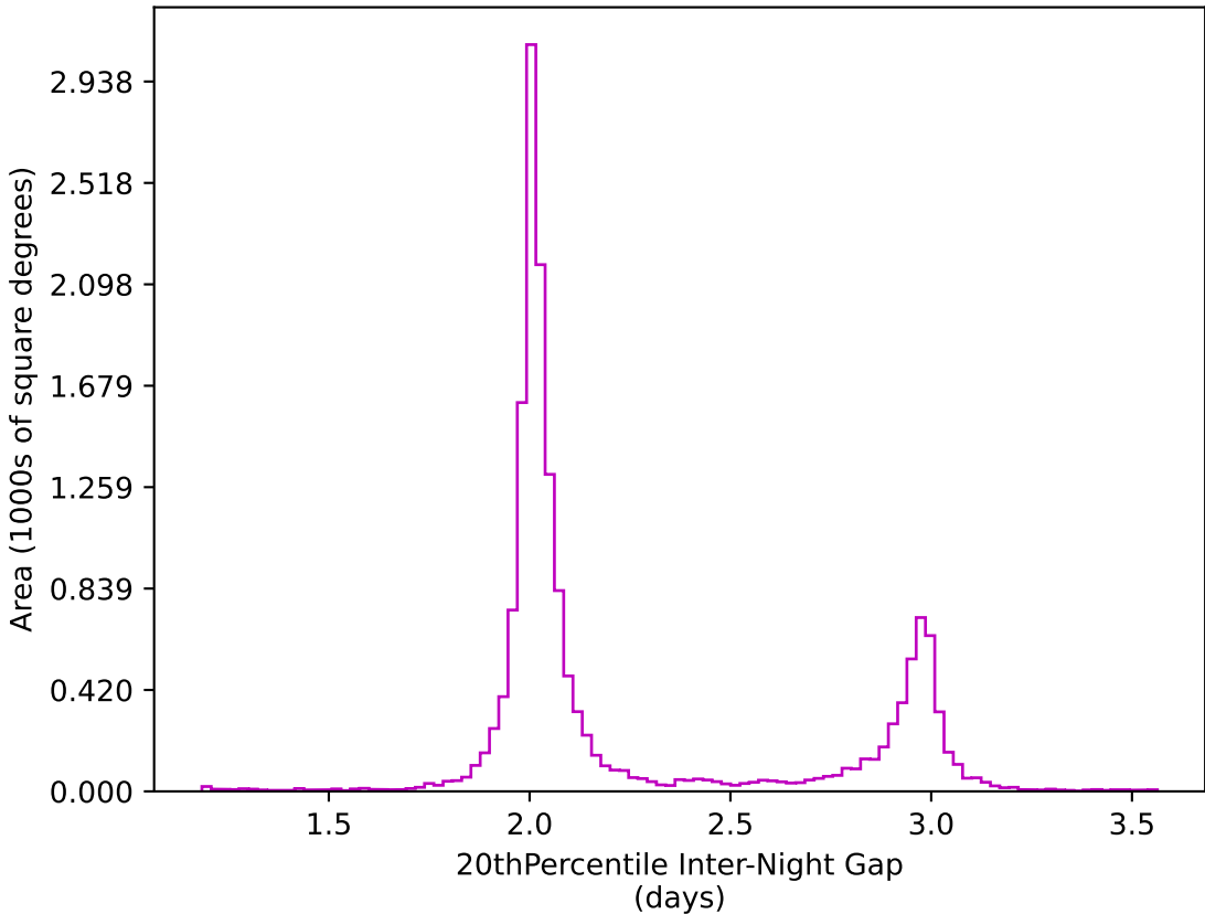
too_100_4v3.4_10yrs WFD z band: 20thPercentile Inter-Night Gap
