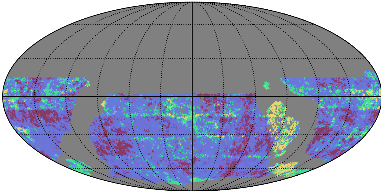
too_100_4v3.4_10yrs WFD y band: 20thPercentile Inter-Night Gap
