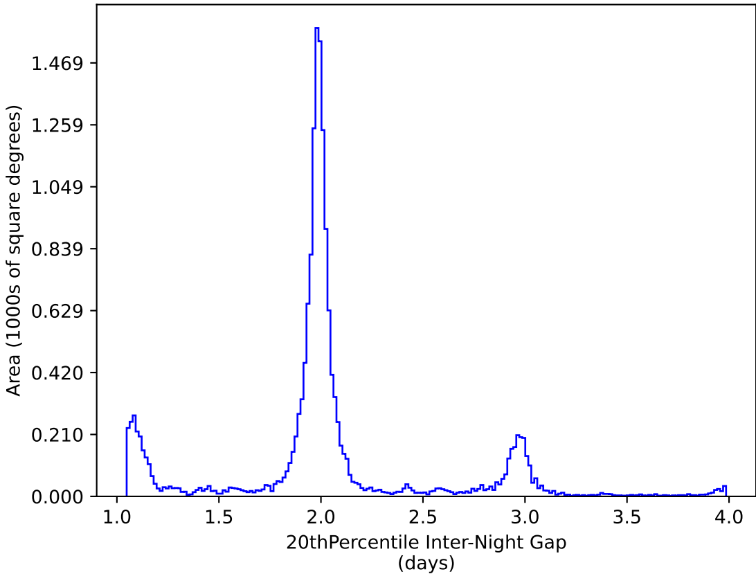
too_100_4v3.4_10yrs WFD y band: 20thPercentile Inter-Night Gap
