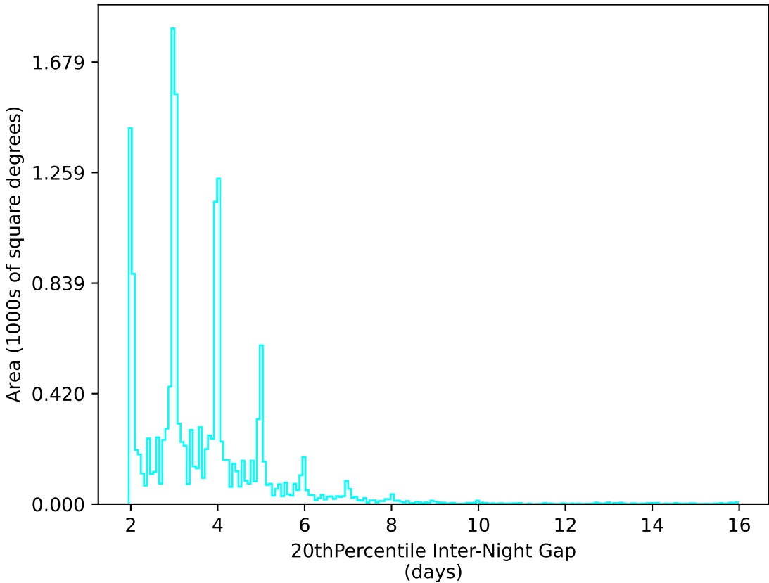
too_100_4v3.4_10yrs WFD u band: 20thPercentile Inter-Night Gap
