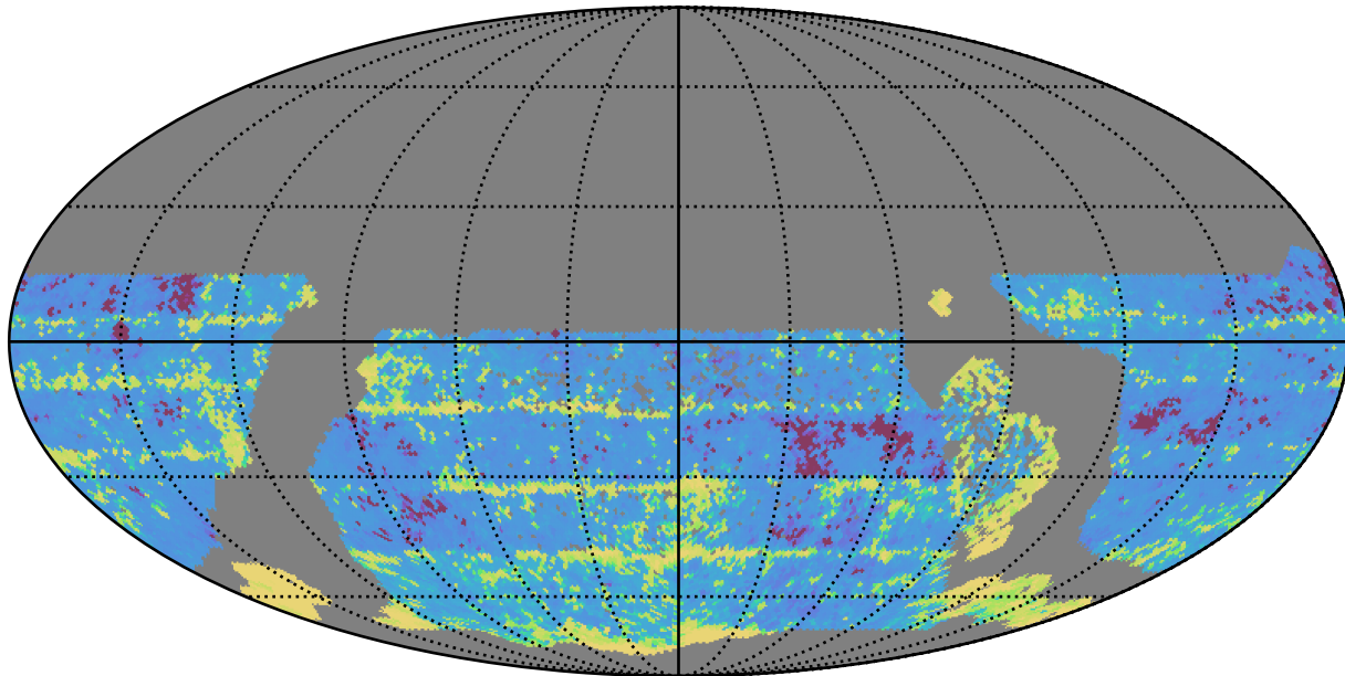
too_100_4v3.4_10yrs WFD i band: 20thPercentile Inter-Night Gap
