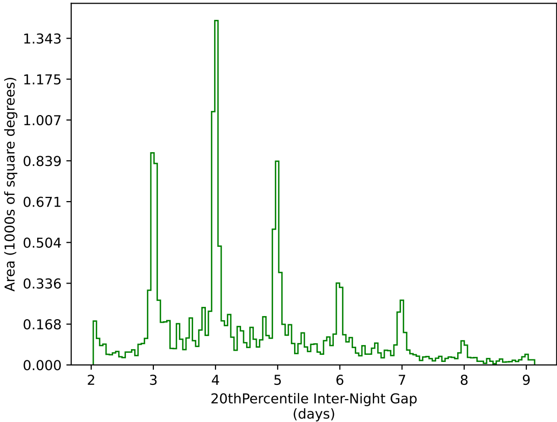
too_100_4v3.4_10yrs WFD g band: 20thPercentile Inter-Night Gap
