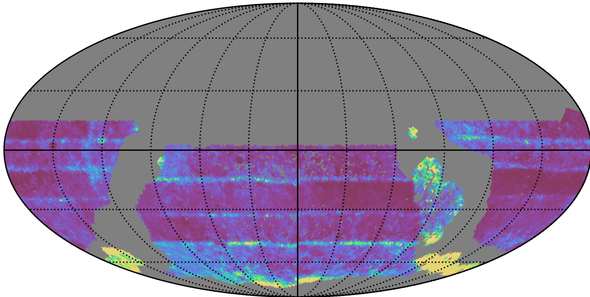
too_100_4v3.4_10yrs WFD all bands: 20thPercentile Inter-Night Gap
