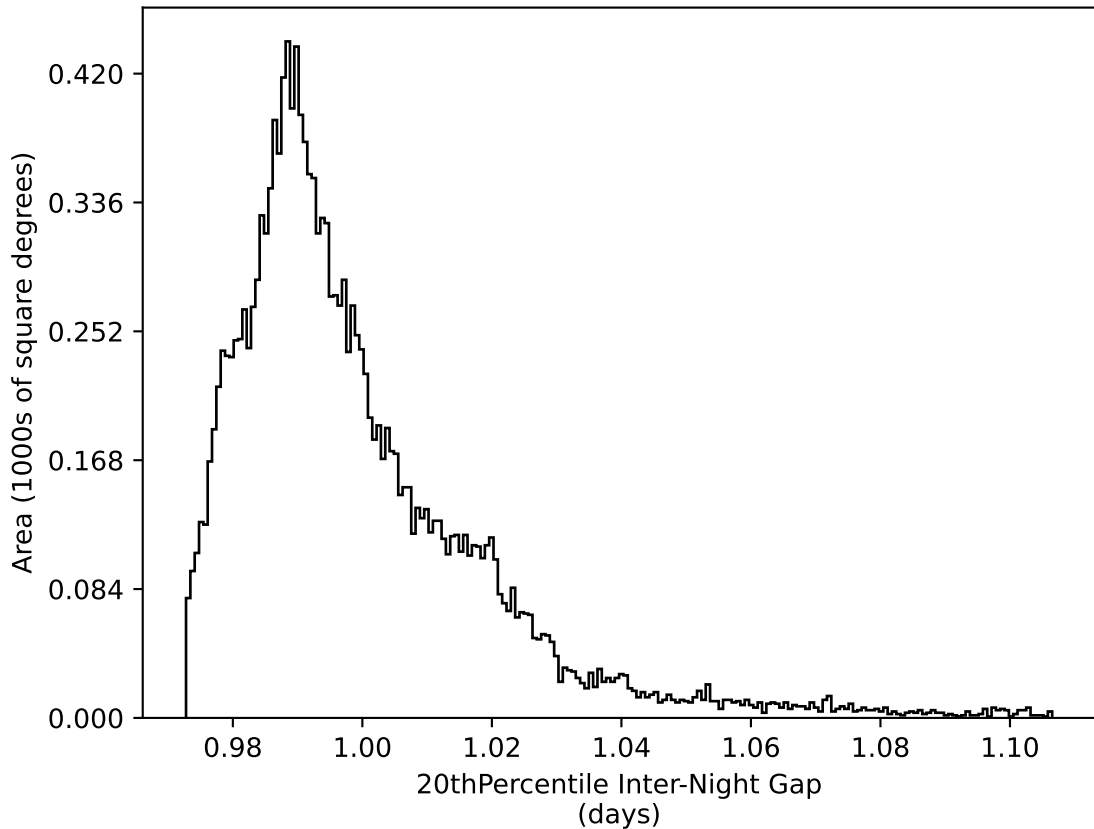
too_100_4v3.4_10yrs WFD all bands: 20thPercentile Inter-Night Gap
