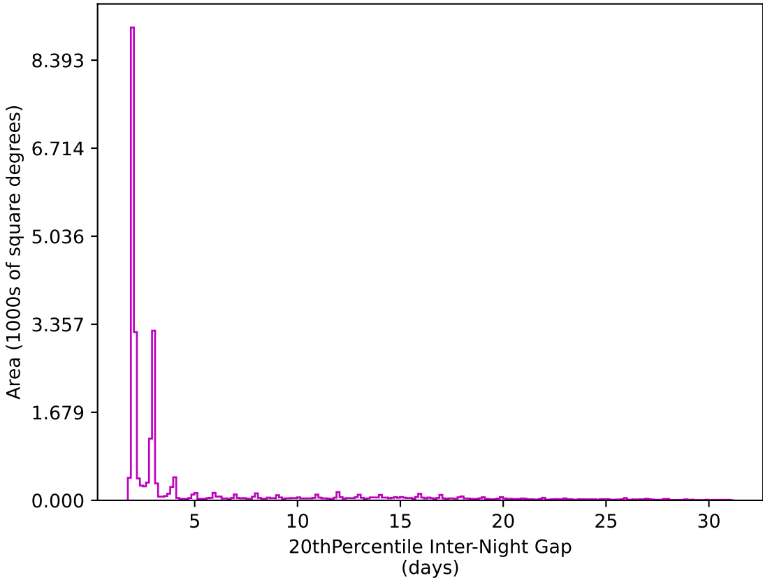
too_100_4v3.4_10yrs All sky z band: 20thPercentile Inter-Night Gap
