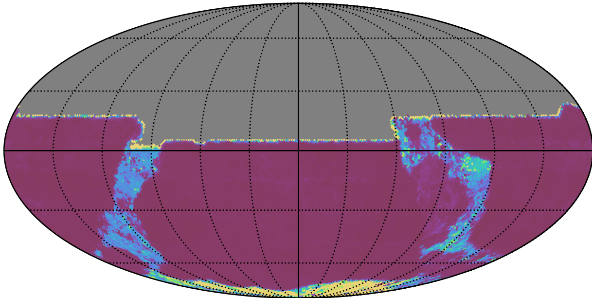
too_100_4v3.4_10yrs All sky y band: 20thPercentile Inter-Night Gap
