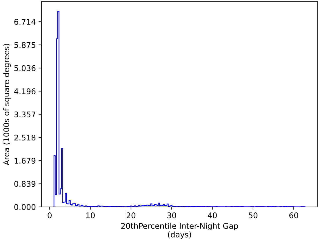
too_100_4v3.4_10yrs All sky y band: 20thPercentile Inter-Night Gap
