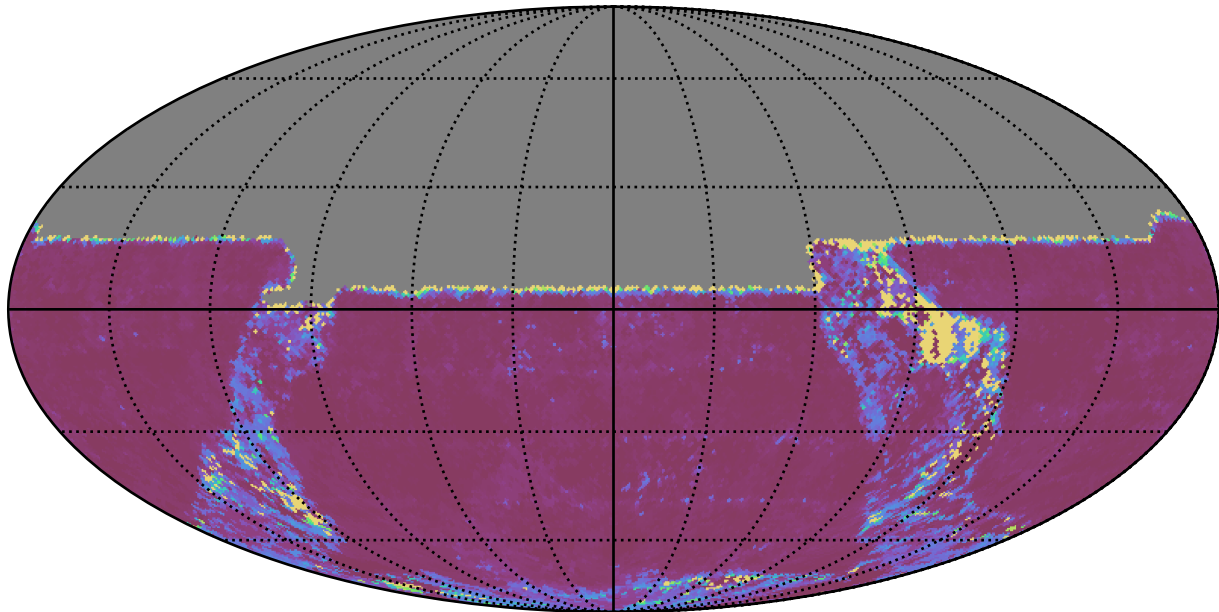
too_100_4v3.4_10yrs All sky u band: 20thPercentile Inter-Night Gap
