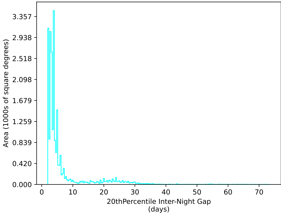
too_100_4v3.4_10yrs All sky u band: 20thPercentile Inter-Night Gap
