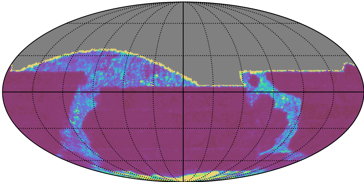
too_100_4v3.4_10yrs All sky r band: 20thPercentile Inter-Night Gap
