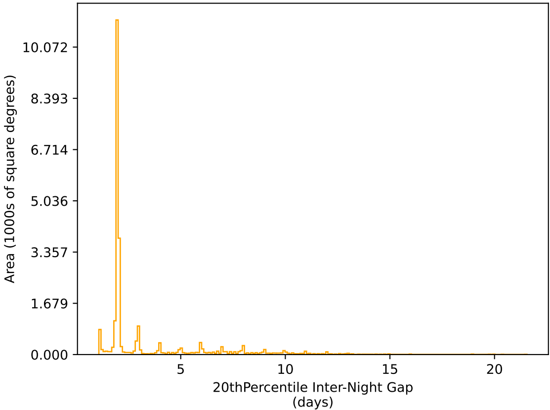
too_100_4v3.4_10yrs All sky r band: 20thPercentile Inter-Night Gap
