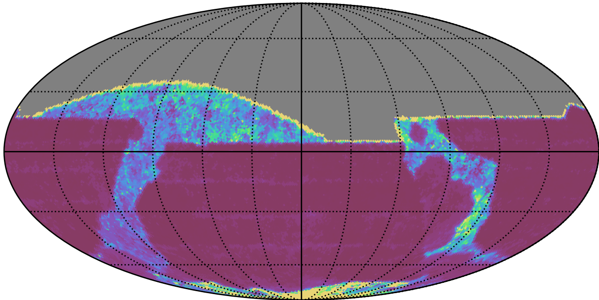
too_100_4v3.4_10yrs All sky i band: 20thPercentile Inter-Night Gap
