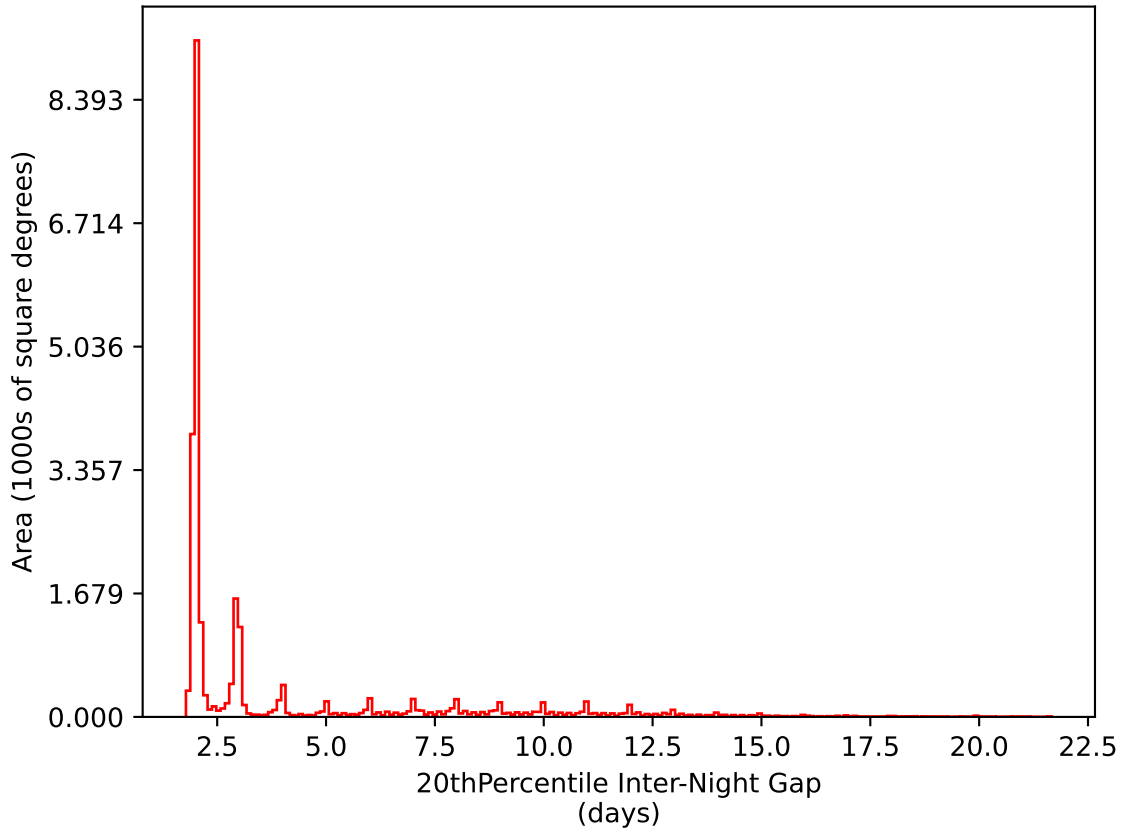
too_100_4v3.4_10yrs All sky i band: 20thPercentile Inter-Night Gap
